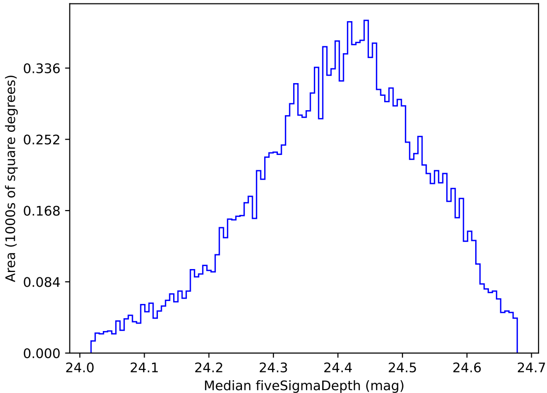
too_elab_r128_d3_gz_v3.4_10yrs WFD g band: Median fiveSigmaDepth
