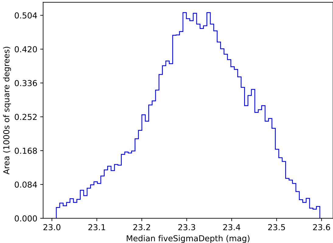
too_elab_r128_d3_gz_v3.4_10yrs WFD all bands: Median fiveSigmaDepth
