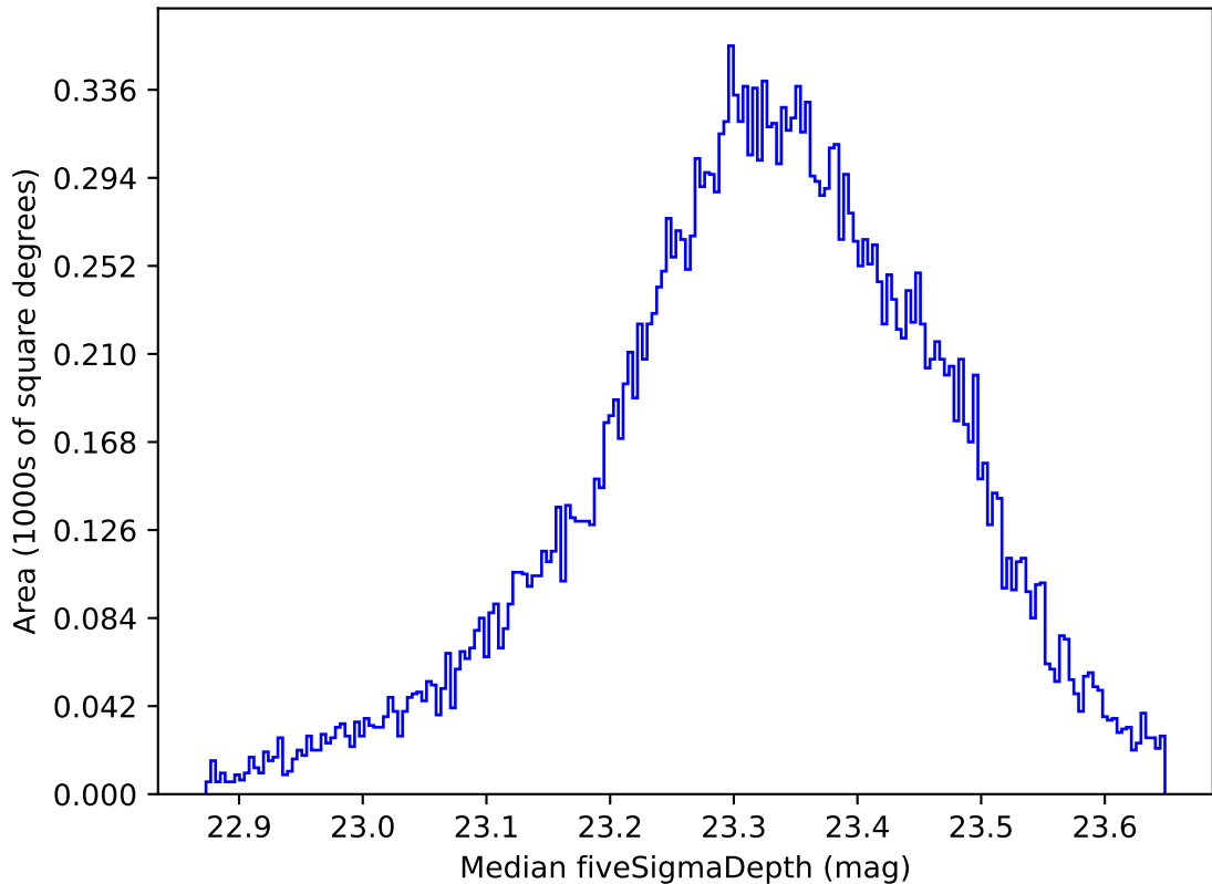
too_elab_r128_d3_gz_v3.4_10yrs All sky all bands: Median fiveSigmaDepth
