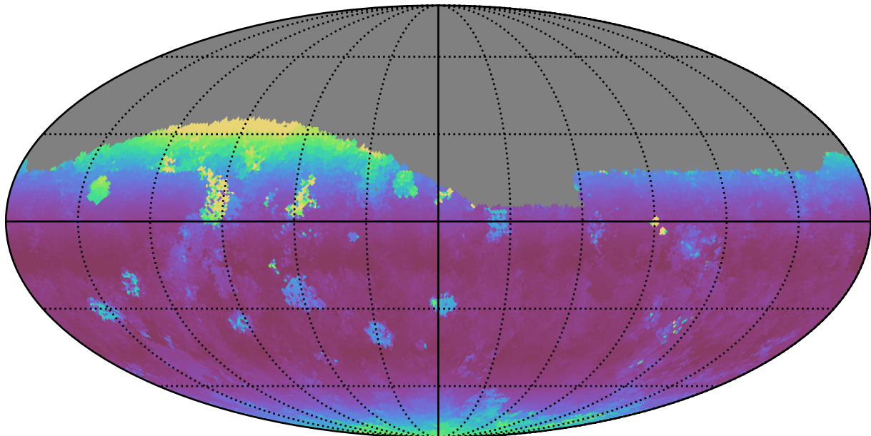
too_elab_r128_d3_gz_v3.4_10yrs Yr 1 z band: Median airmass
