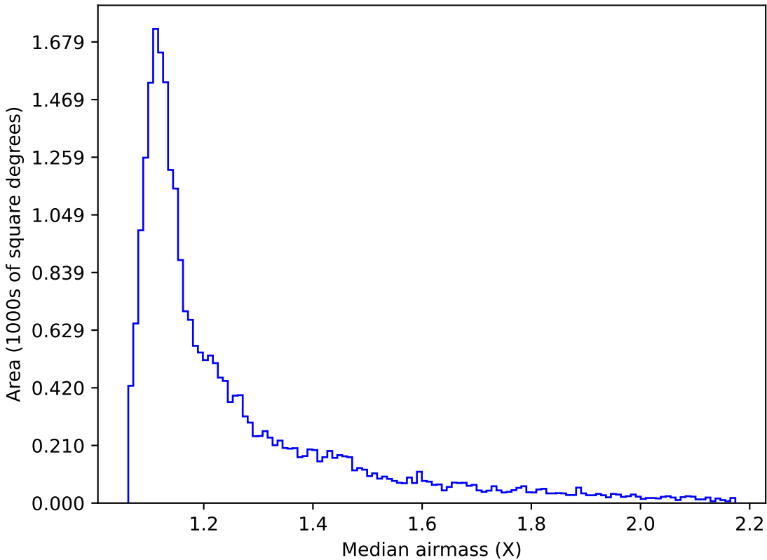
too_elab_r128_d3_gz_v3.4_10yrs Yr 1 z band: Median airmass
