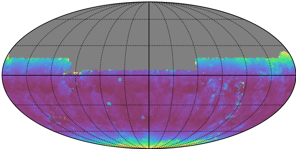
too_elab_r128_d3_gz_v3.4_10yrs Yr 1 y band: Median airmass
