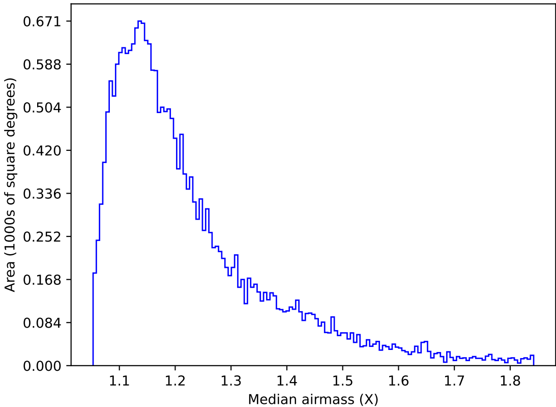
too_elab_r128_d3_gz_v3.4_10yrs Yr 1 u band: Median airmass
