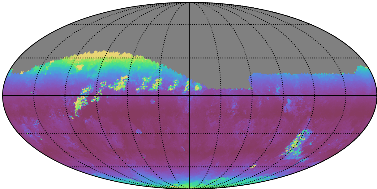
too_elab_r128_d3_gz_v3.4_10yrs Yr 1 r band: Median airmass
