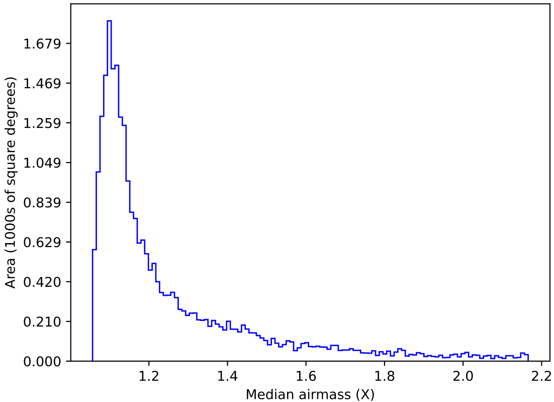
too_elab_r128_d3_gz_v3.4_10yrs Yr 1 r band: Median airmass
