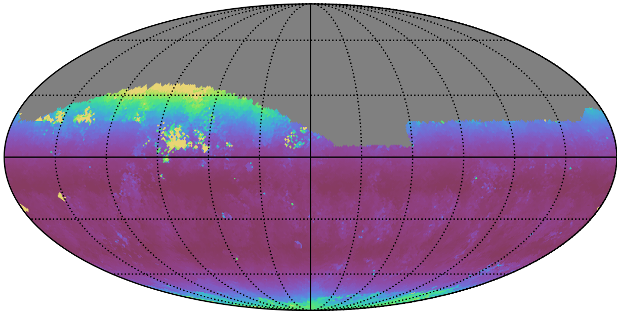
too_elab_r128_d3_gz_v3.4_10yrs Yr 1 i band: Median airmass
