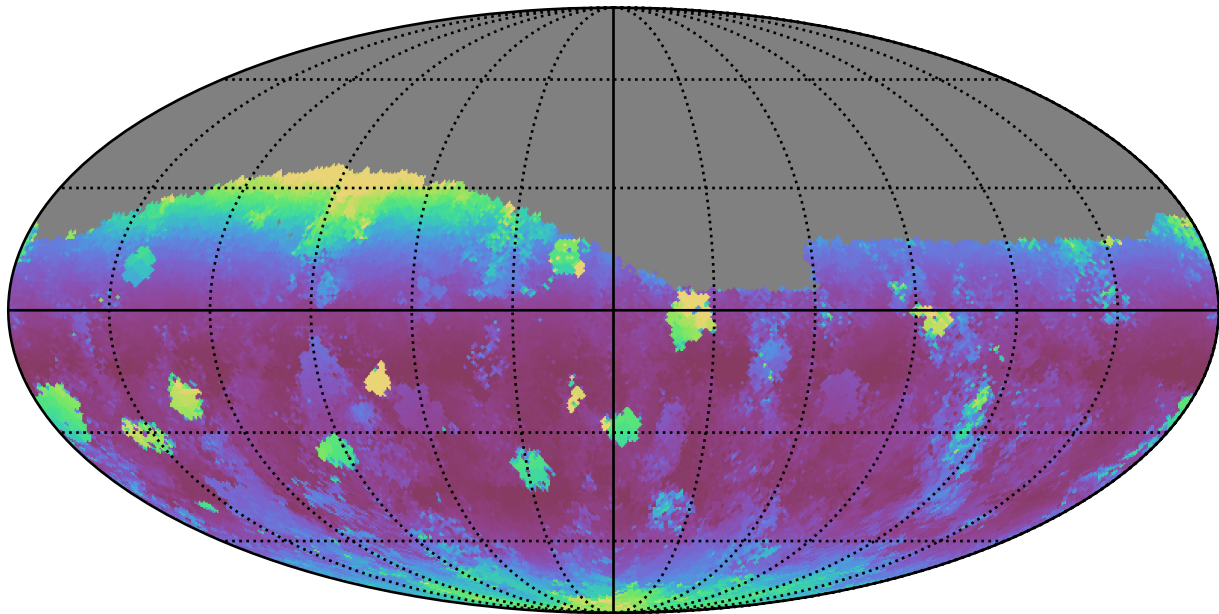
too_elab_r128_d3_gz_v3.4_10yrs Yr 1 g band: Median airmass
