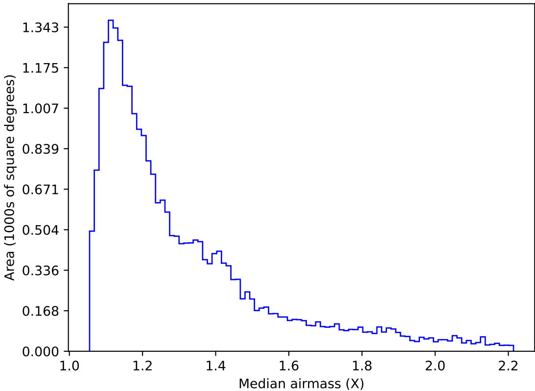
too_elab_r128_d3_gz_v3.4_10yrs Yr 1 g band: Median airmass
