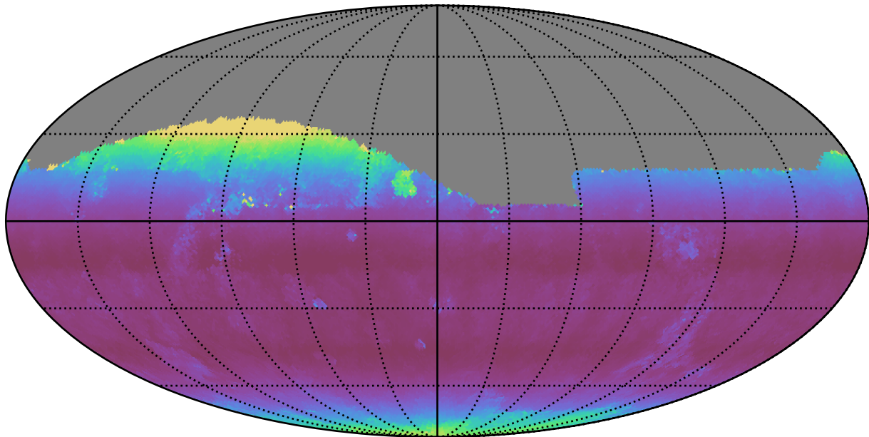
too_elab_r128_d3_gz_v3.4_10yrs Yr 1 all bands: Median airmass
