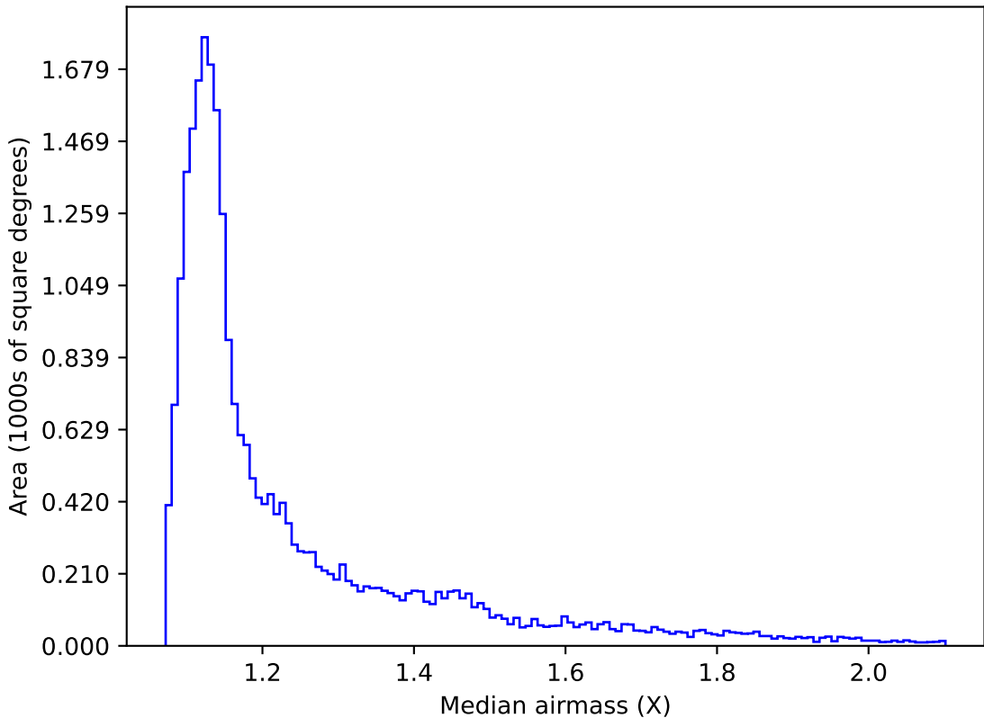
too_elab_r128_d3_gz_v3.4_10yrs Yr 1 all bands: Median airmass
