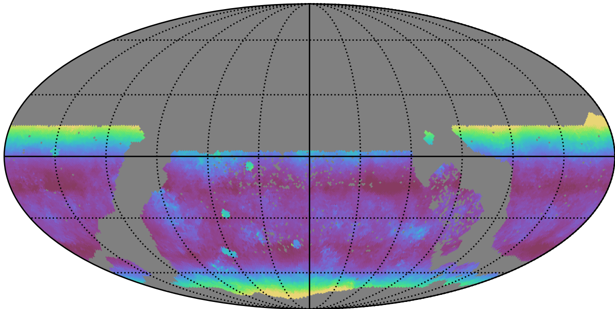
too_elab_r128_d3_gz_v3.4_10yrs WFD z band: Median airmass
