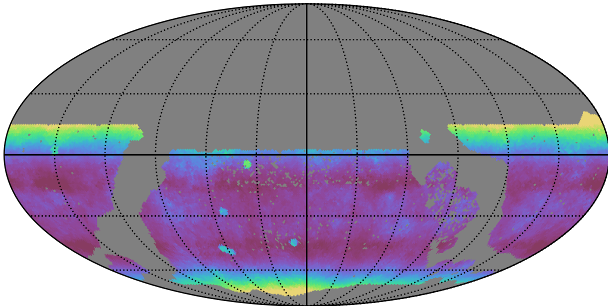
too_elab_r128_d3_gz_v3.4_10yrs WFD y band: Median airmass
