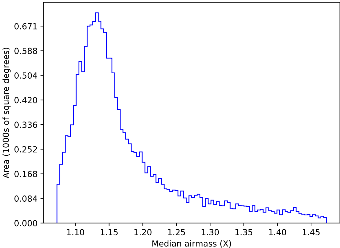
too_elab_r128_d3_gz_v3.4_10yrs WFD u band: Median airmass
