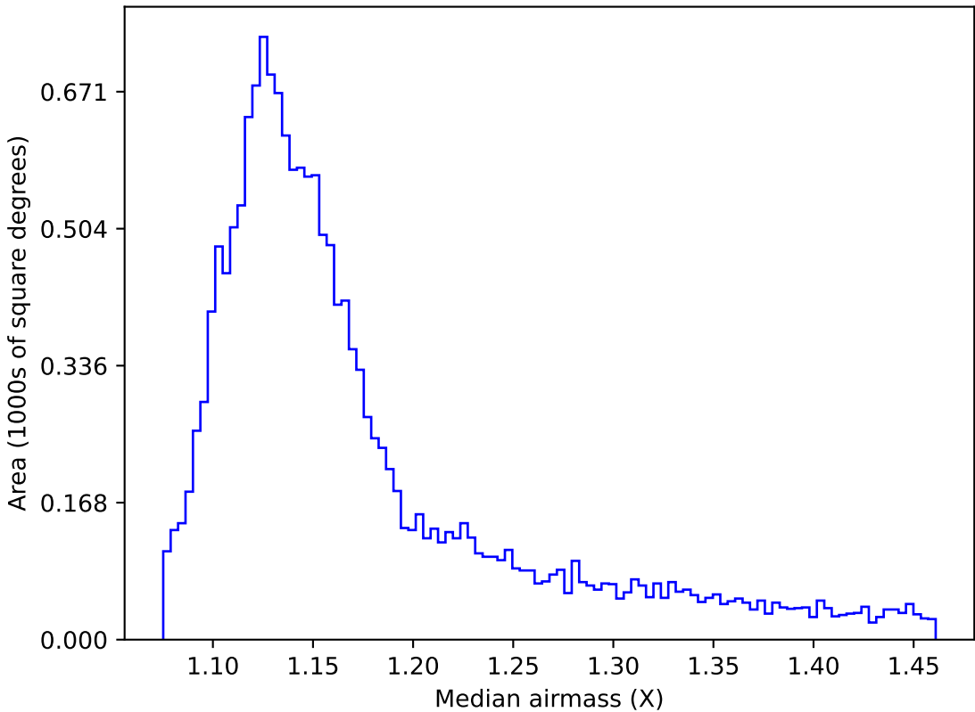
too_elab_r128_d3_gz_v3.4_10yrs WFD r band: Median airmass
