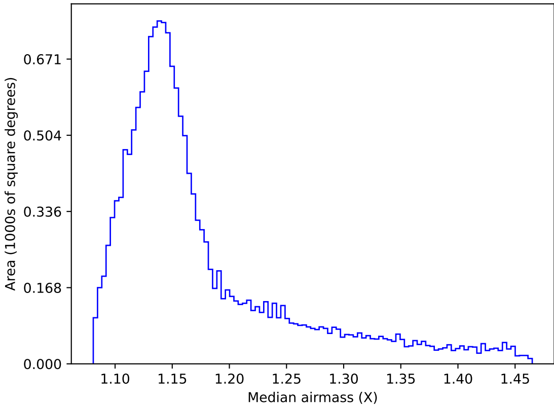
too_elab_r128_d3_gz_v3.4_10yrs WFD i band: Median airmass
