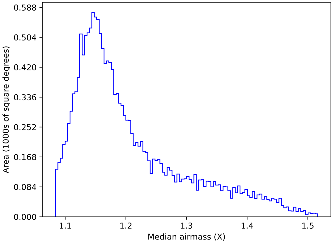
too_elab_r128_d3_gz_v3.4_10yrs WFD g band: Median airmass
