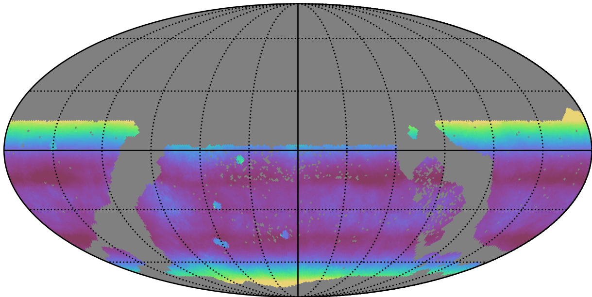
too_elab_r128_d3_gz_v3.4_10yrs WFD all bands: Median airmass
