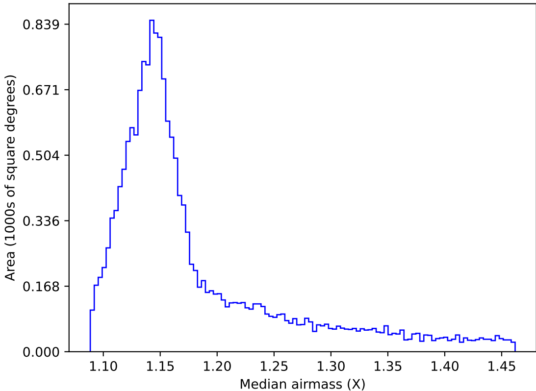
too_elab_r128_d3_gz_v3.4_10yrs WFD all bands: Median airmass
