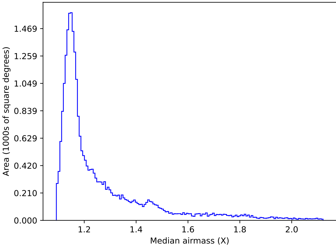
too_elab_r128_d3_gz_v3.4_10yrs All sky z band: Median airmass
