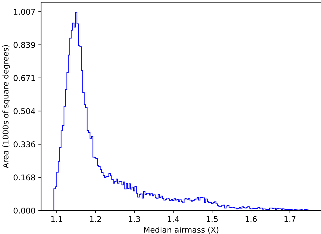
too_elab_r128_d3_gz_v3.4_10yrs All sky y band: Median airmass
