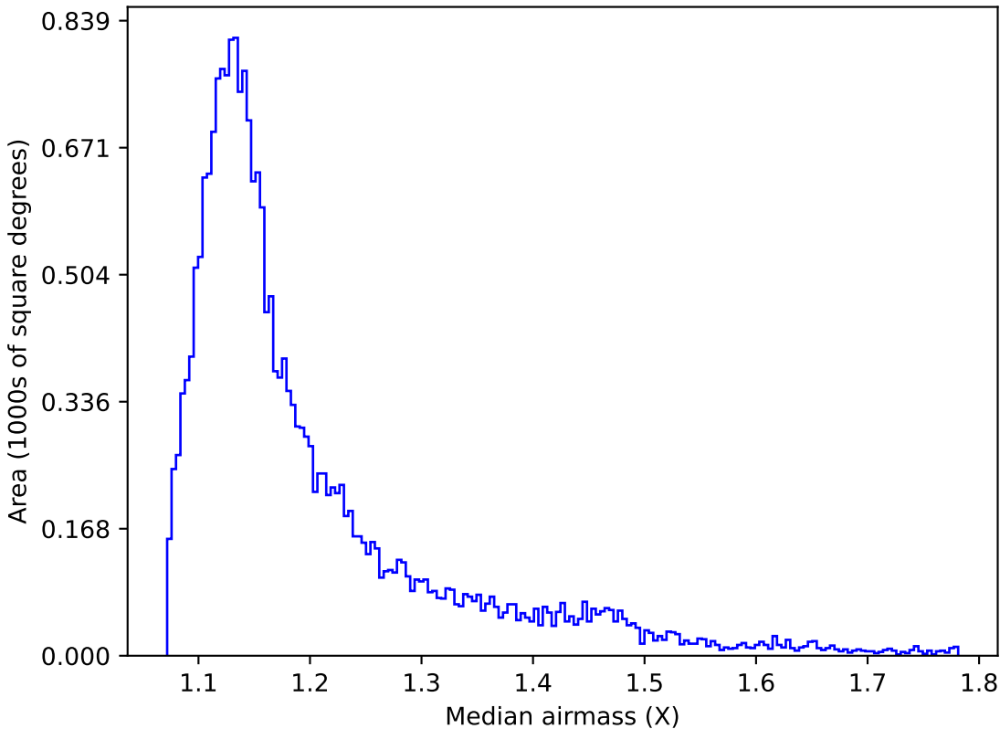
too_elab_r128_d3_gz_v3.4_10yrs All sky u band: Median airmass
