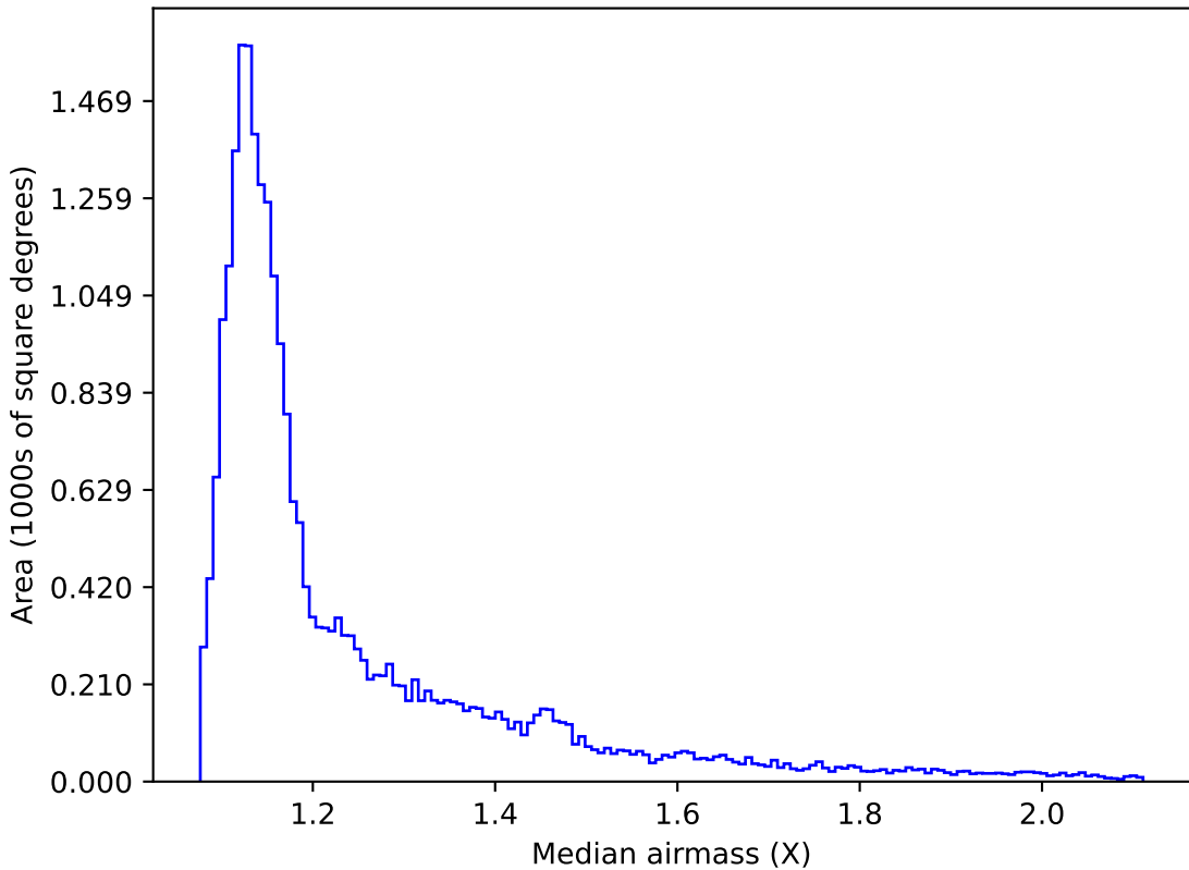
too_elab_r128_d3_gz_v3.4_10yrs All sky r band: Median airmass
