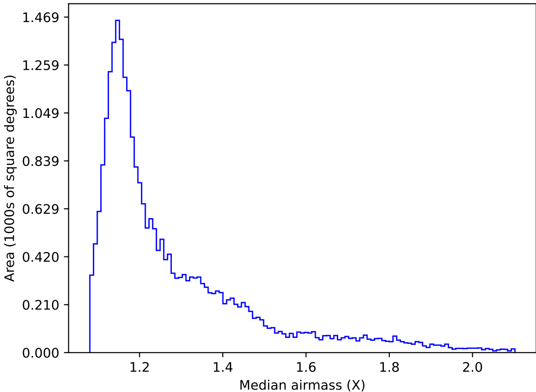
too_elab_r128_d3_gz_v3.4_10yrs All sky g band: Median airmass
