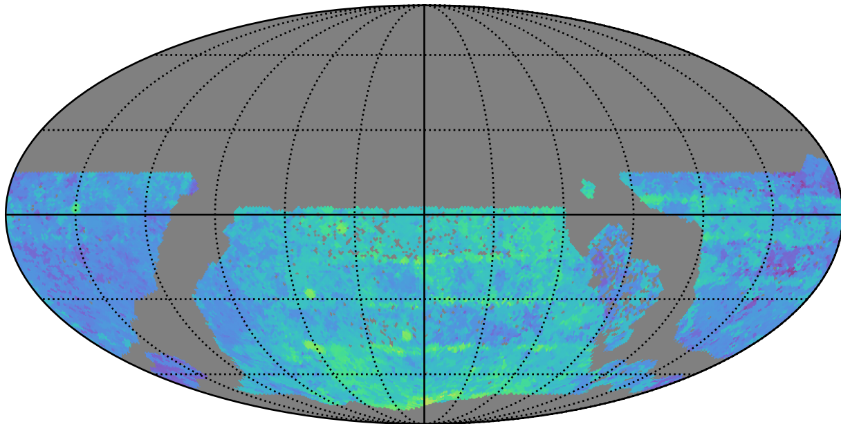
too_elab_r128_d3_gz_v3.4_10yrs WFD y band: Median Season Length
