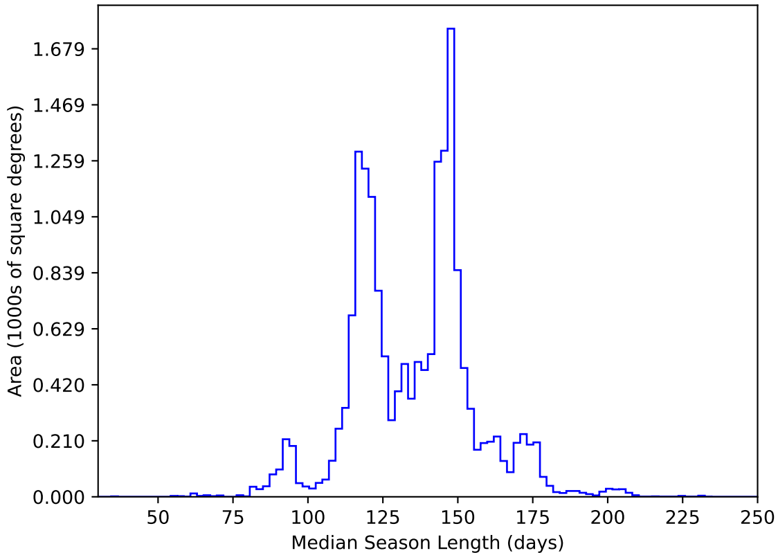
too_elab_r128_d3_gz_v3.4_10yrs WFD y band: Median Season Length
