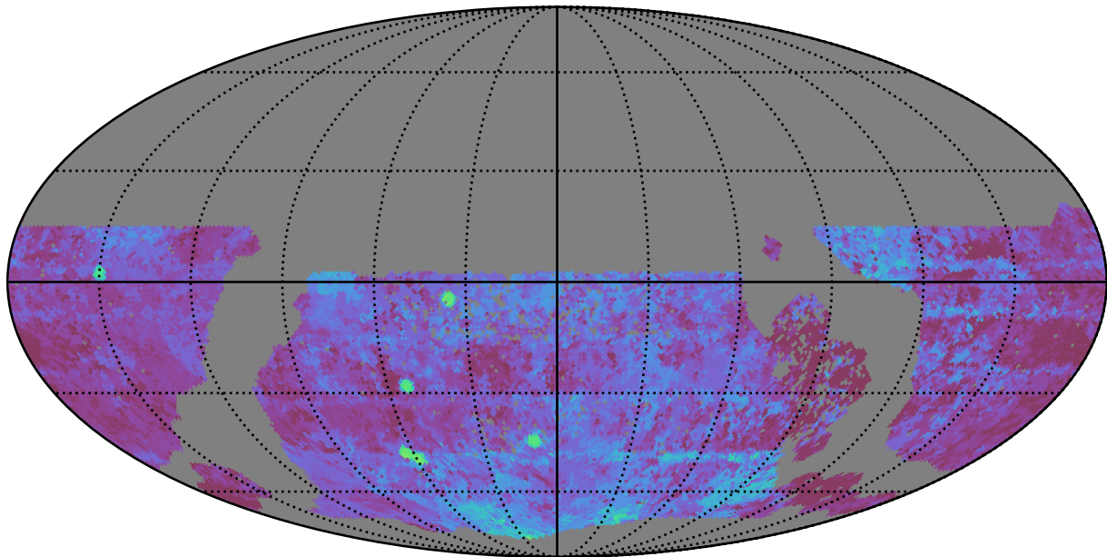
too_elab_r128_d3_gz_v3.4_10yrs WFD u band: Median Season Length
