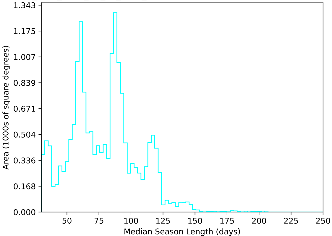
too_elab_r128_d3_gz_v3.4_10yrs WFD u band: Median Season Length
