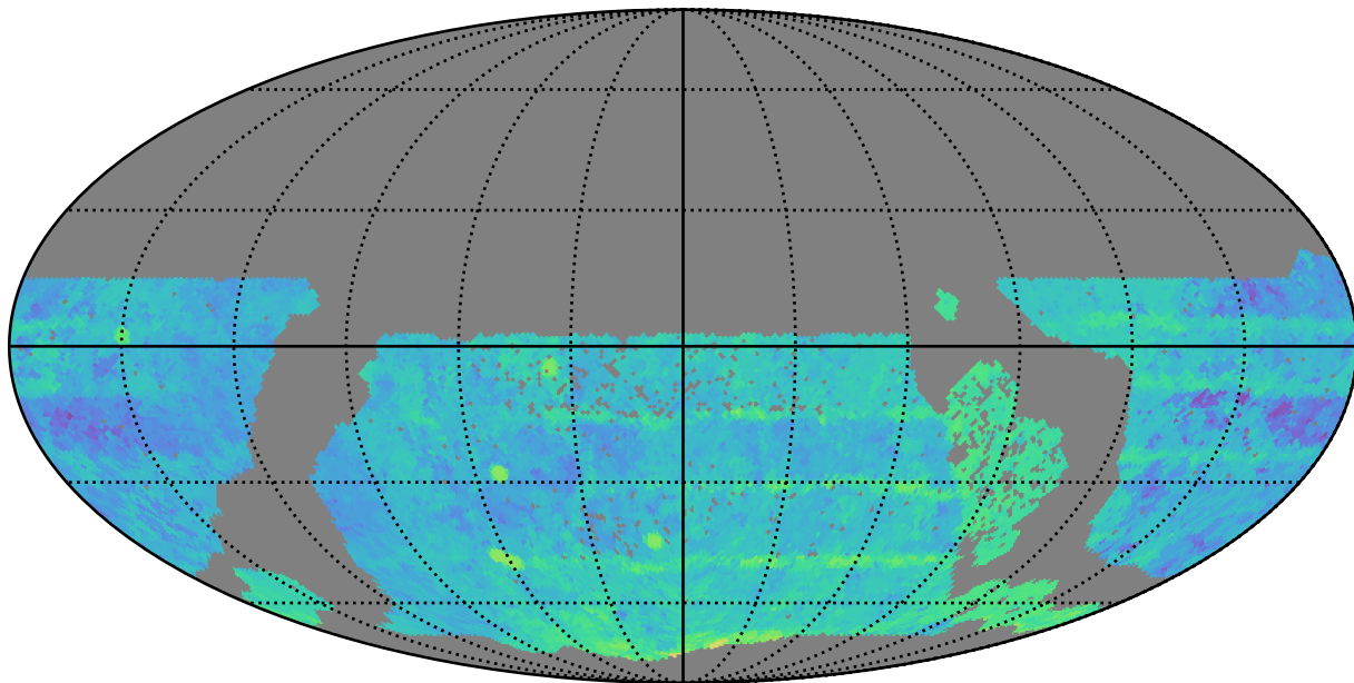
too_elab_r128_d3_gz_v3.4_10yrs WFD r band: Median Season Length
