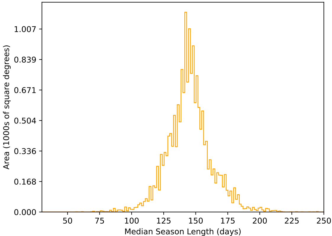
too_elab_r128_d3_gz_v3.4_10yrs WFD r band: Median Season Length
