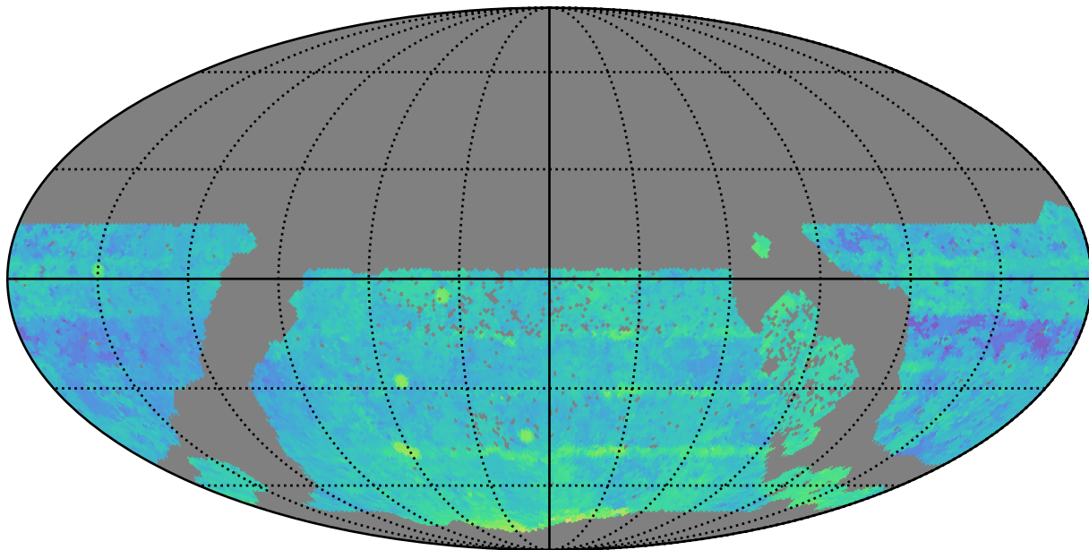
too_elab_r128_d3_gz_v3.4_10yrs WFD i band: Median Season Length
