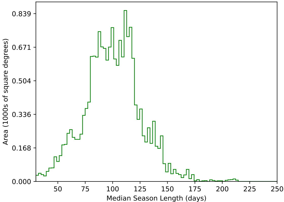
too_elab_r128_d3_gz_v3.4_10yrs WFD g band: Median Season Length
