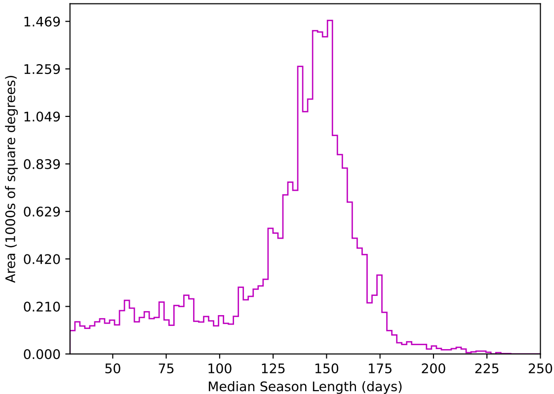
too_elab_r128_d3_gz_v3.4_10yrs All sky z band: Median Season Length
