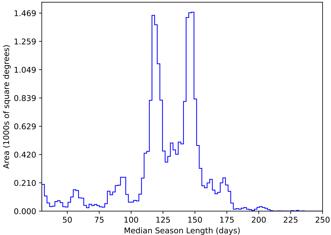
too_elab_r128_d3_gz_v3.4_10yrs All sky y band: Median Season Length
