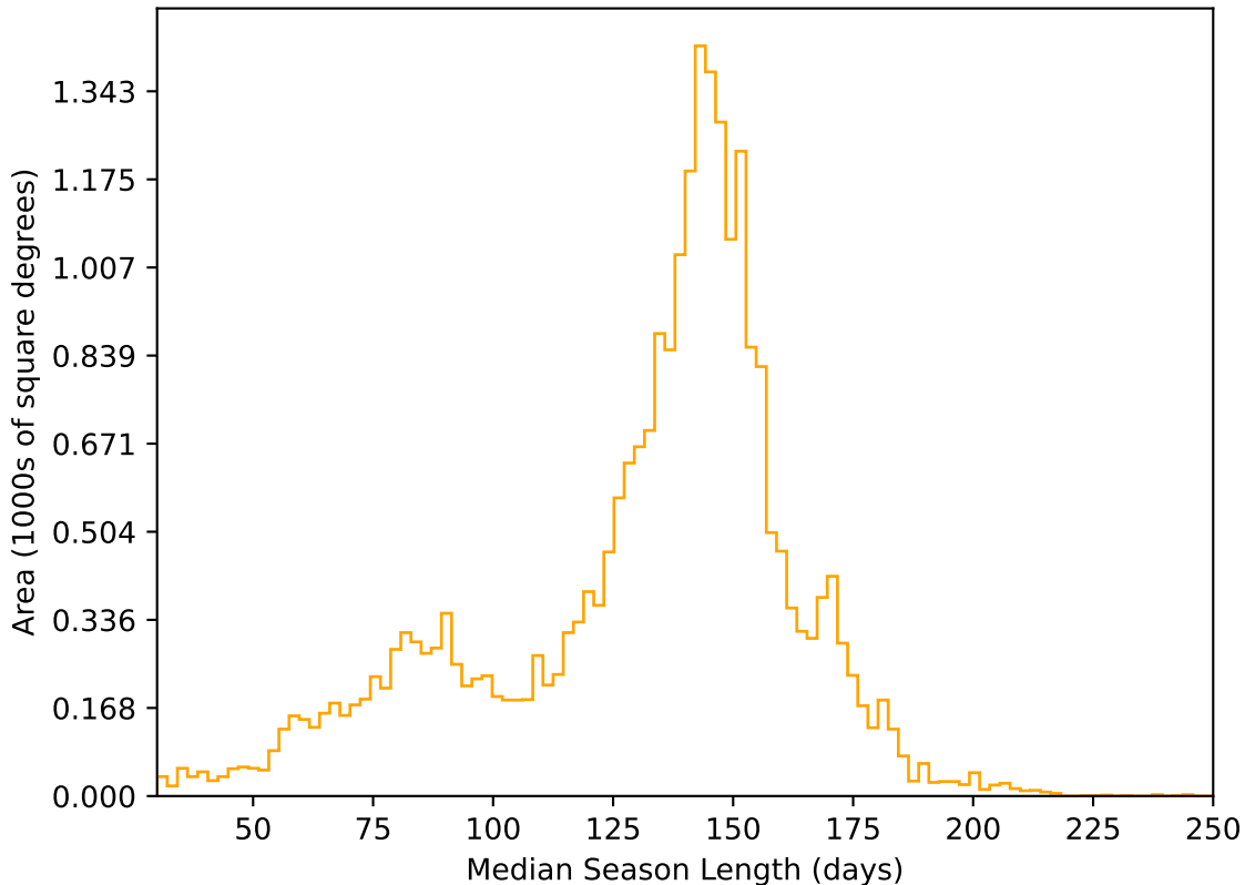
too_elab_r128_d3_gz_v3.4_10yrs All sky r band: Median Season Length
