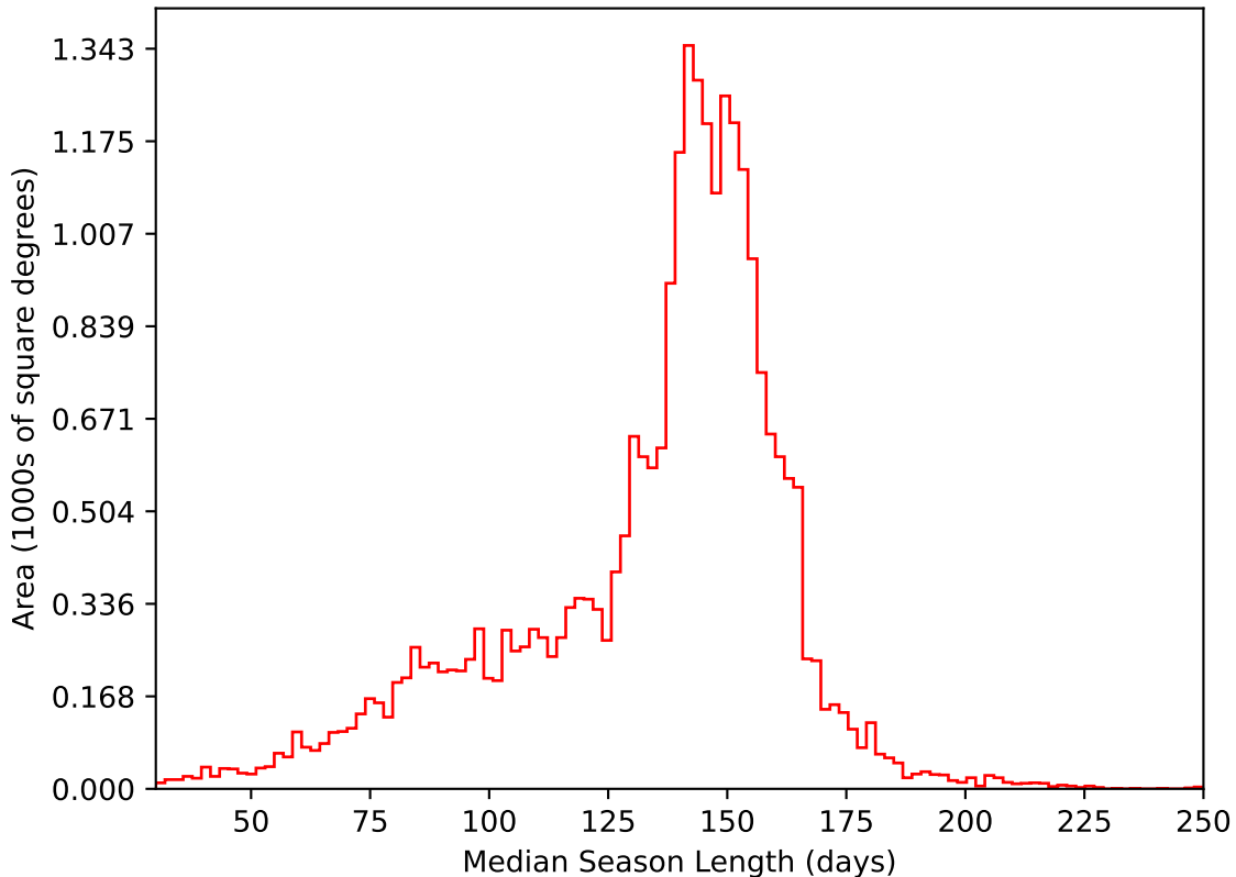
too_elab_r128_d3_gz_v3.4_10yrs All sky i band: Median Season Length
