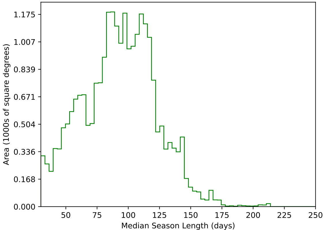
too_elab_r128_d3_gz_v3.4_10yrs All sky g band: Median Season Length
