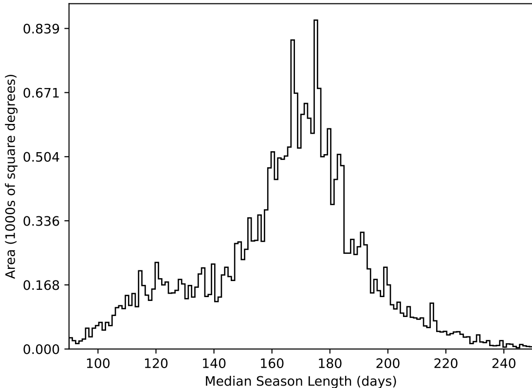
too_elab_r128_d3_gz_v3.4_10yrs All sky all bands: Median Season Length
