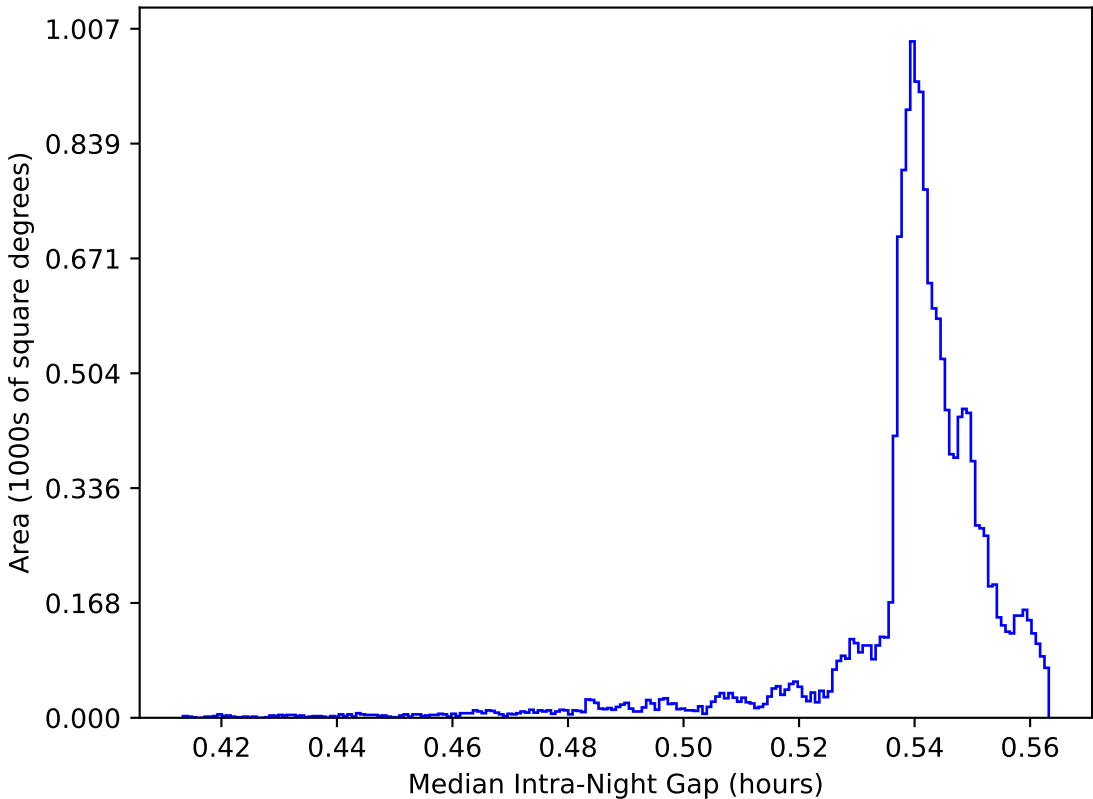
too_elab_r128_d3_gz_v3.4_10yrs WFD: Median Intra-Night Gap
