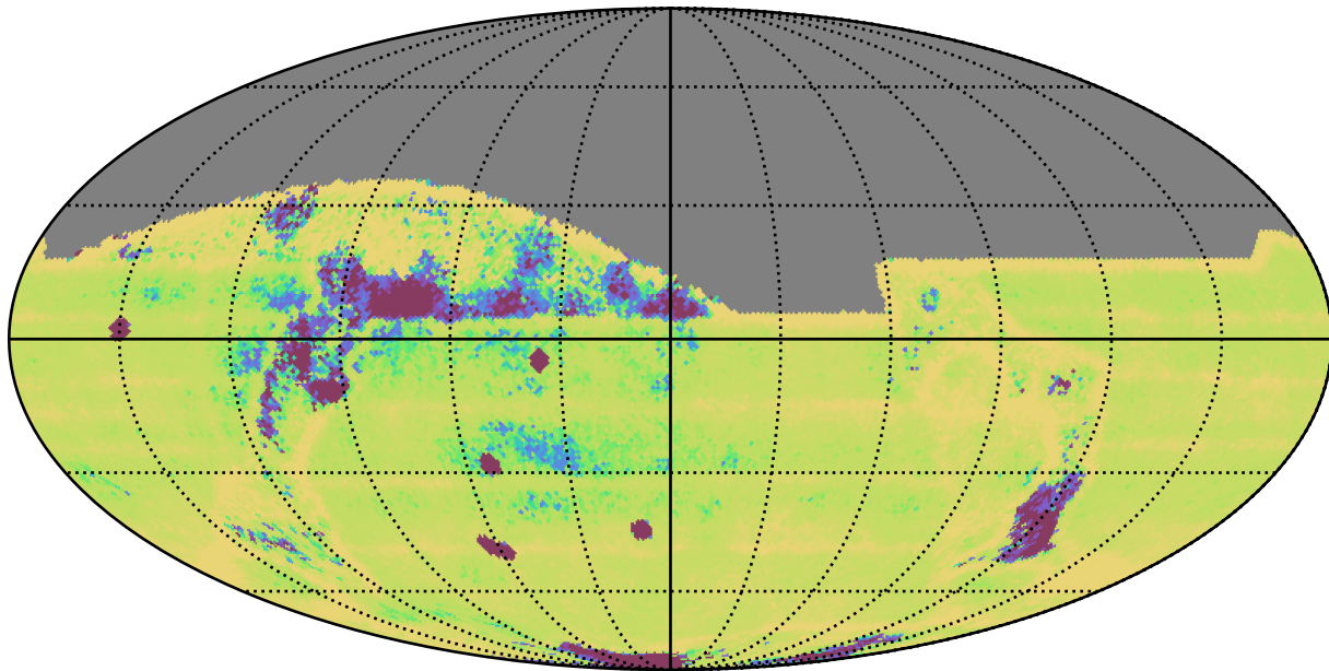
too_elab_r128_d3_gz_v3.4_10yrs All sky: Median Intra-Night Gap
