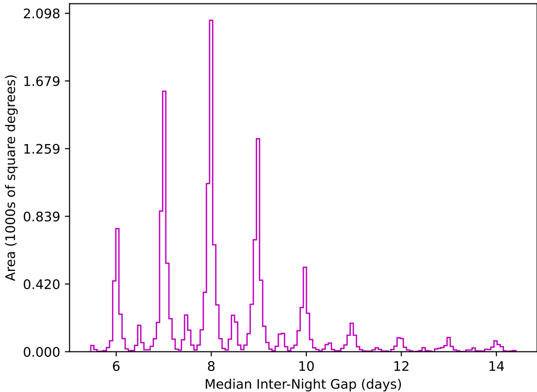
too_elab_r128_d3_gz_v3.4_10yrs WFD z band: Median Inter-Night Gap
