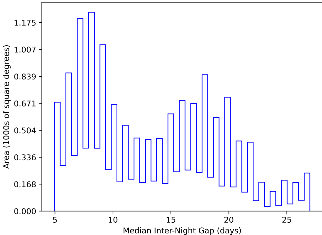
too_elab_r128_d3_gz_v3.4_10yrs WFD y band: Median Inter-Night Gap
