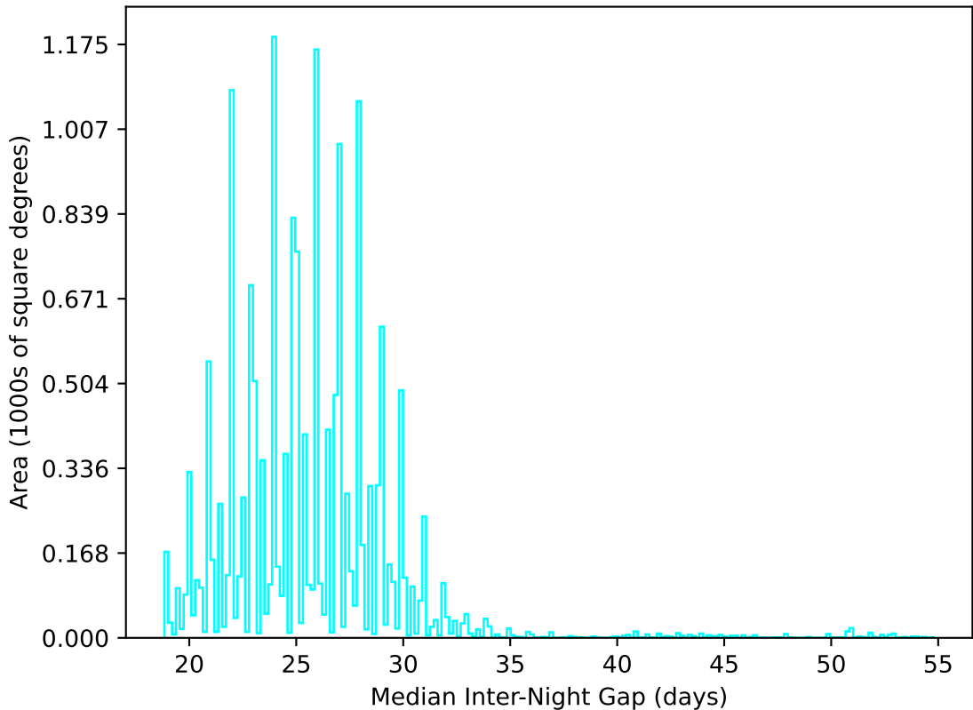
too_elab_r128_d3_gz_v3.4_10yrs WFD u band: Median Inter-Night Gap
