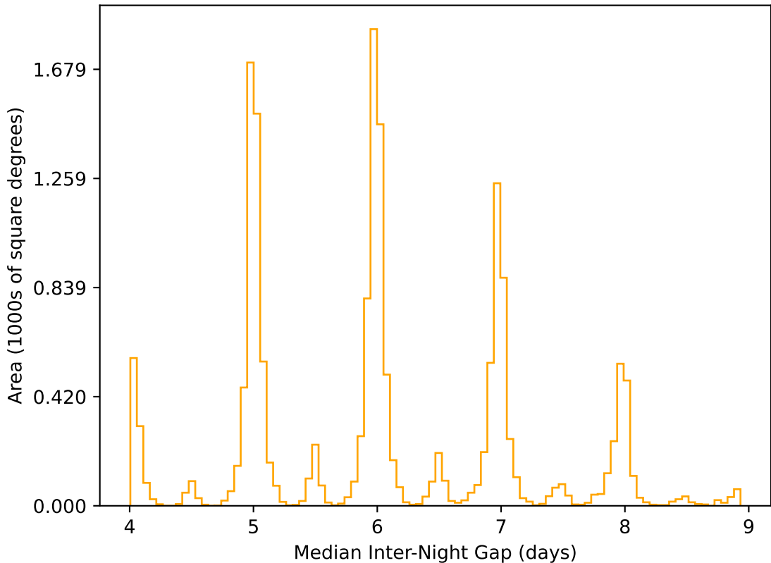
too_elab_r128_d3_gz_v3.4_10yrs WFD r band: Median Inter-Night Gap
