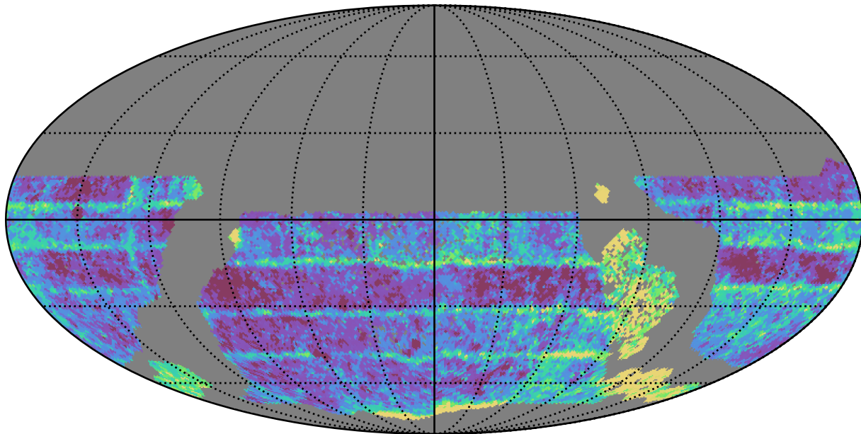
too_elab_r128_d3_gz_v3.4_10yrs WFD i band: Median Inter-Night Gap
