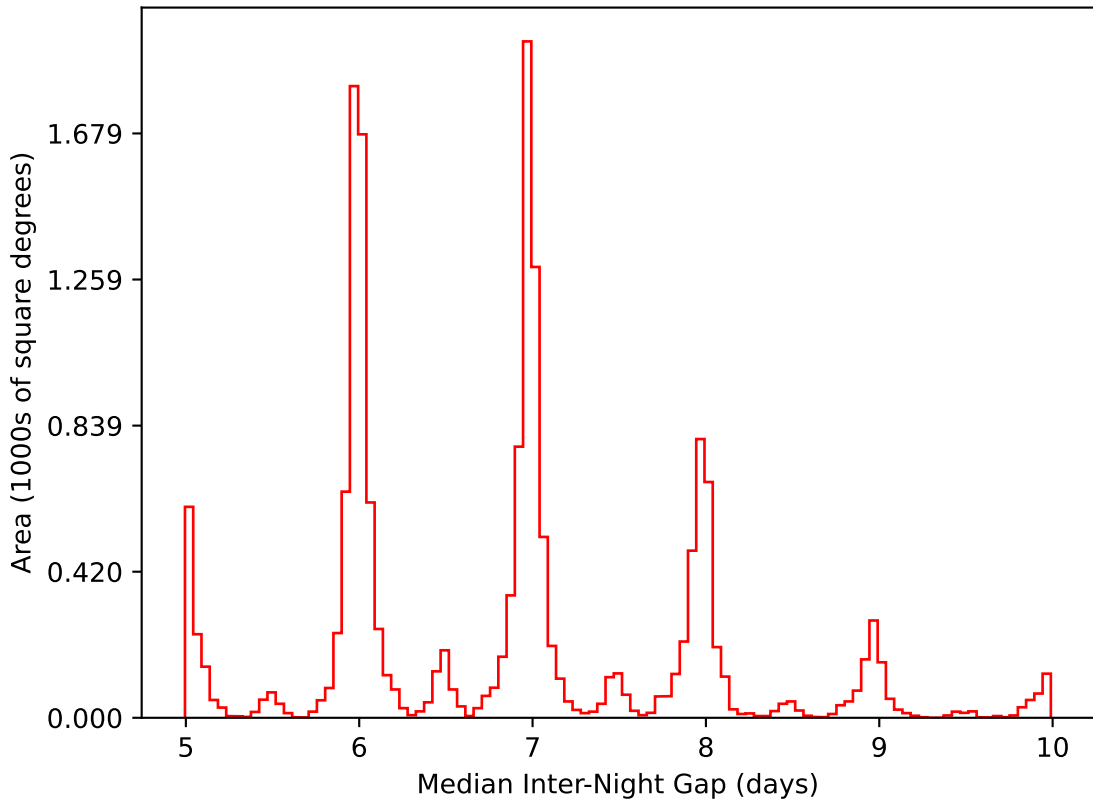
too_elab_r128_d3_gz_v3.4_10yrs WFD i band: Median Inter-Night Gap
