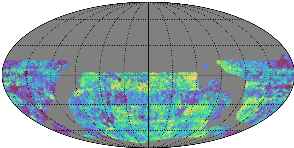
too_elab_r128_d3_gz_v3.4_10yrs WFD g band: Median Inter-Night Gap
